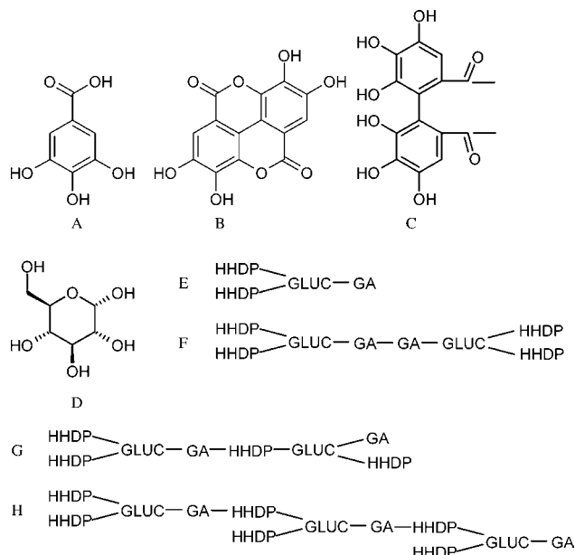
Figure 2. Structures of some ellagitannins and their subunits. (A) Gallic acid, (B) ellagic acid, (C) hexahydroxydiphenoyl unit, (D) D(+)-glucose, (E) casuarictin, (F) agrimoniin, (G) sanguiniin H-6, and (H) lambertianin C. GA, gallic acid; Gluc, glucose; HHDP, hexahydroxydiphenoyl.
